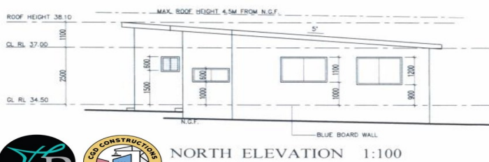
NORTH ELEVATION 1:100
